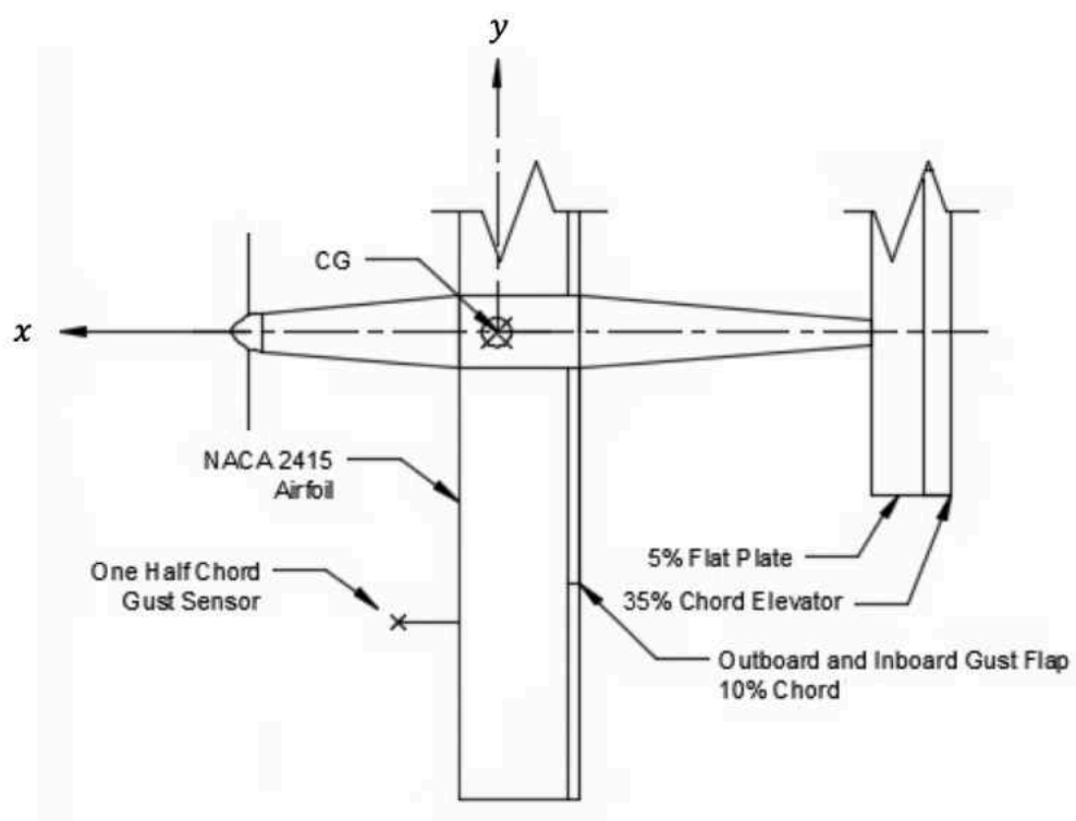
Figure 2.3 ARIS Planform
